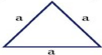
Equilateral Triangle
