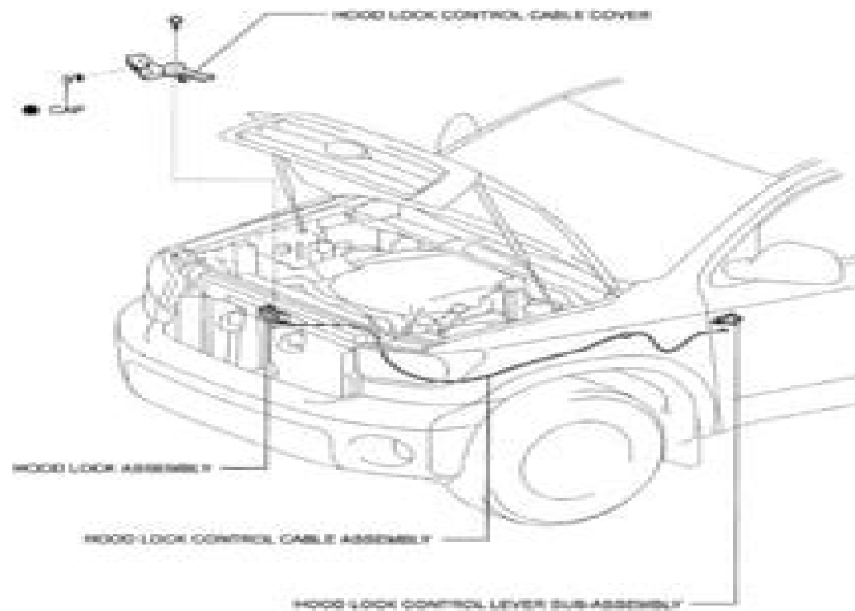
Fig. 13: Identifying Hood Lock Control Cable Assembly Replacement Components (1 Of 3) Courtesy of TOYOTA MOTOR SALES, U.S.A., INC.
