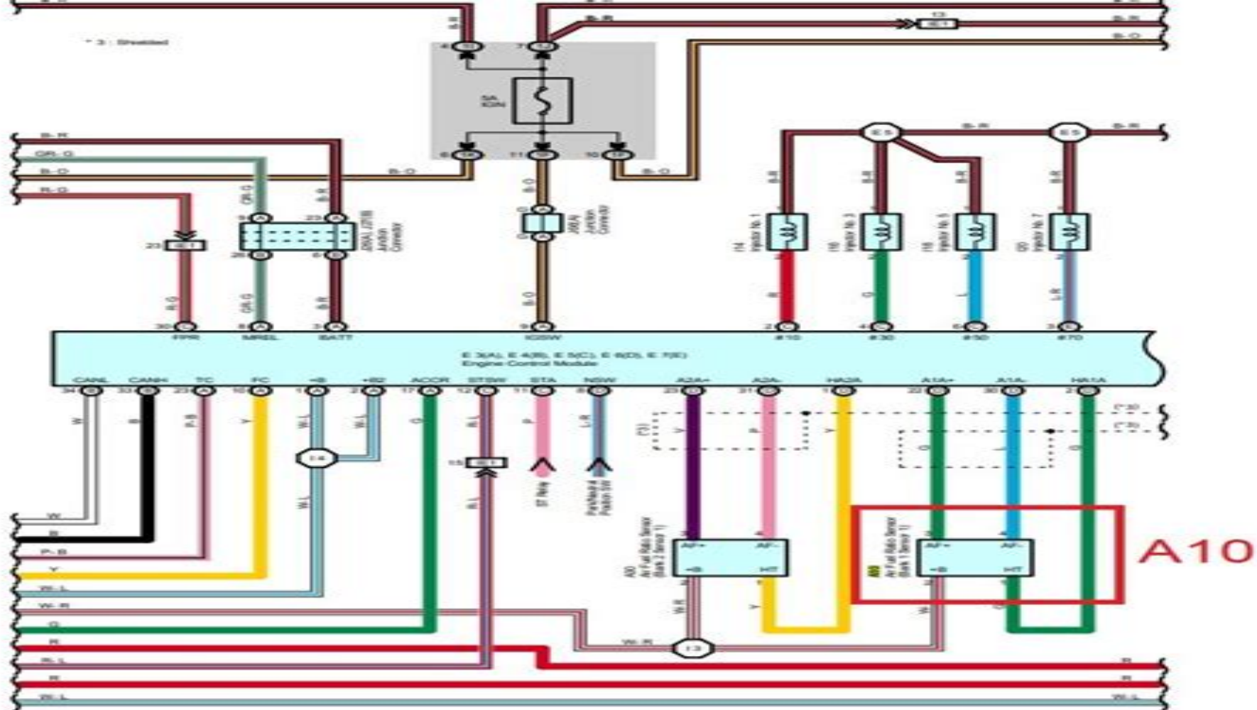
2005 TOYOTA TUNDRA (EWD611U)
