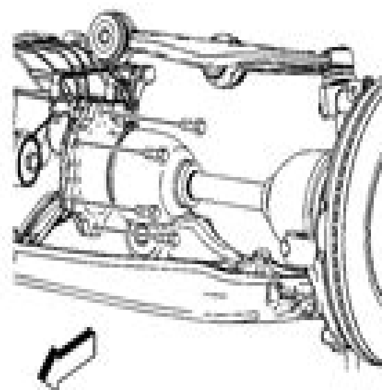
Fig. 9 View Of Wheel Drive Shaft Retaining Bolts Courtesy of GENERAL MOTORS CORP.
