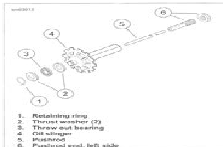
Figure 6-36. Pushrod Assembly: Cable Clutch
