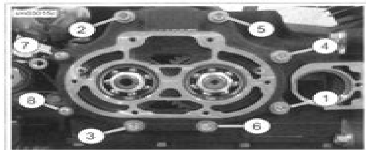
Figure 6-34. Torque Sequence
