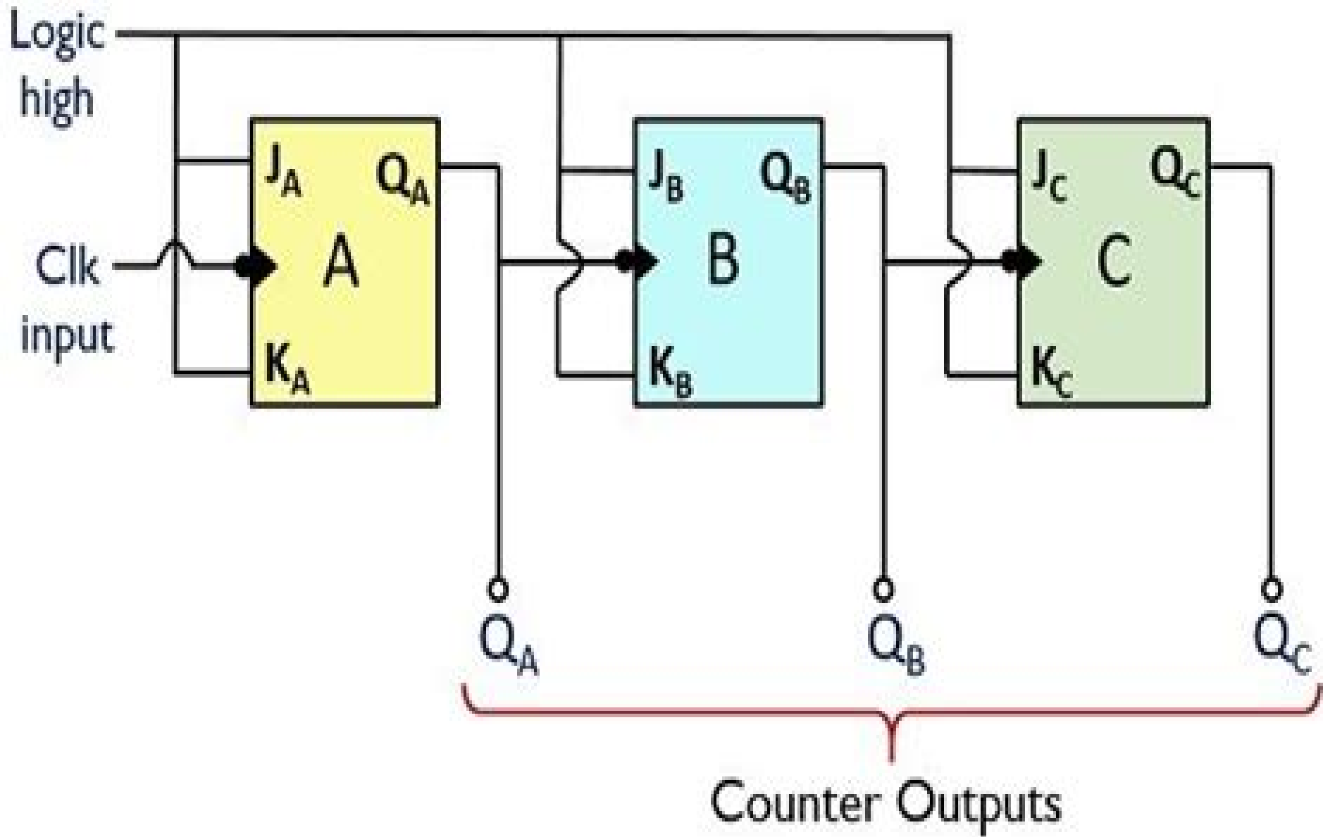
Circuit Diagram of 3-bit Asynchronous Counter
