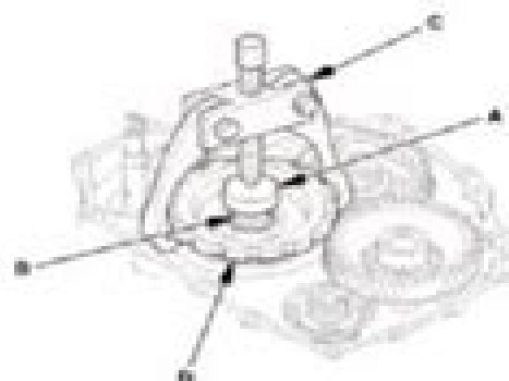
Fig. 116: Setting Commercially Available Bearing Puller On Park Gear Courtesy of AMERICAN HONDA MOTOR CO., INC.
