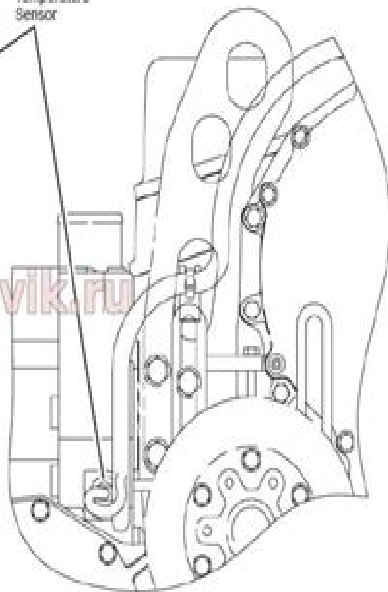
3406E Front View
