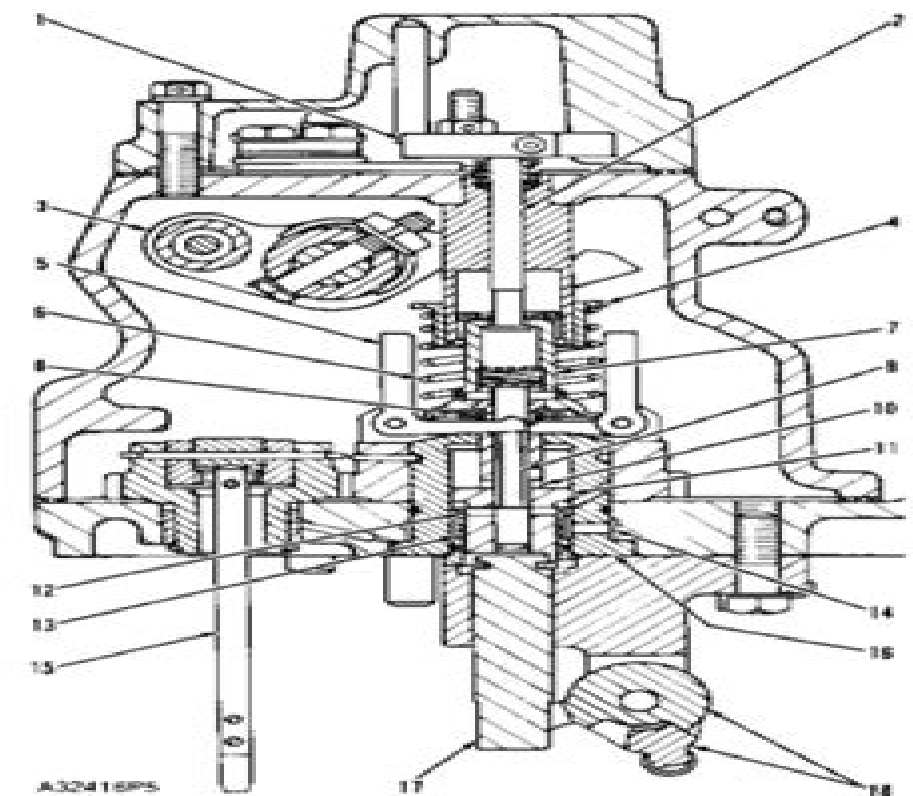
Hydra-Mechanical Governor For Standard Engines (Earlier)
