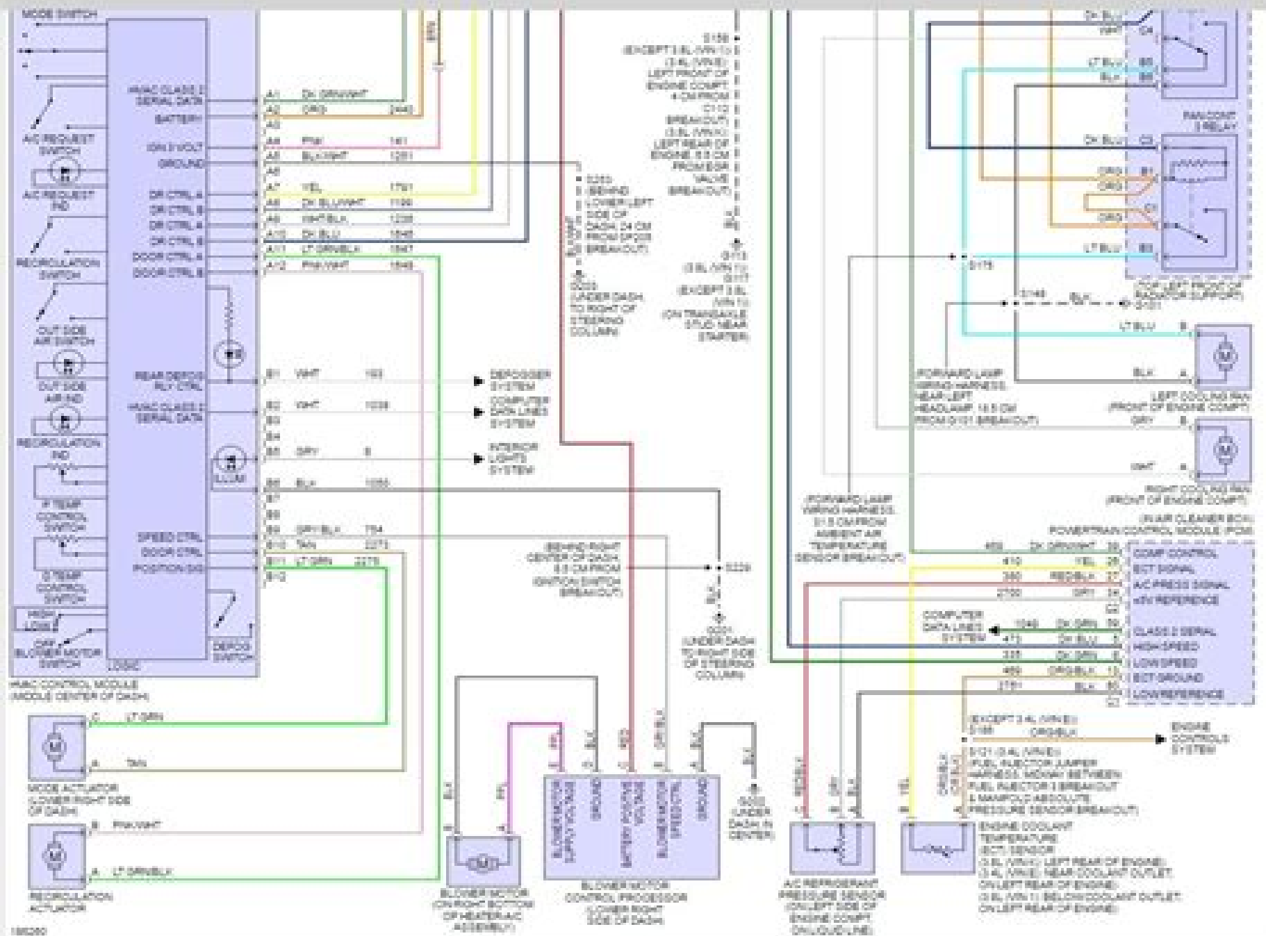
Fig 2: Manual A/C Circuit
