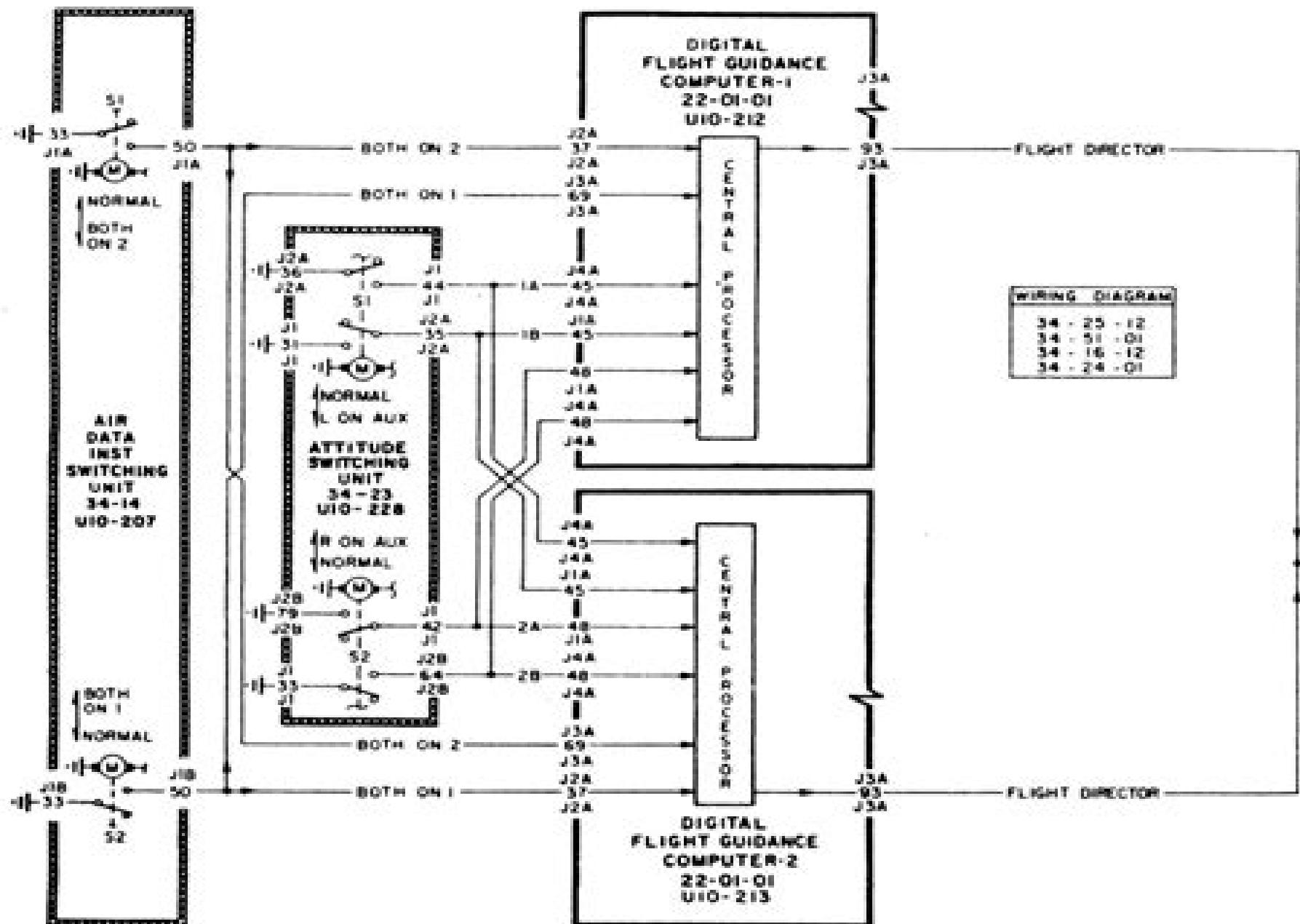
Figure 2-21. Wiring diagram.
