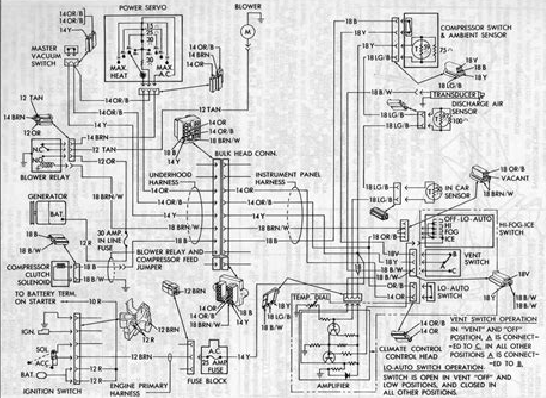
Fig. 1-19 Automatic Climate Control Circuit Diagram (Except 693 & 697)
