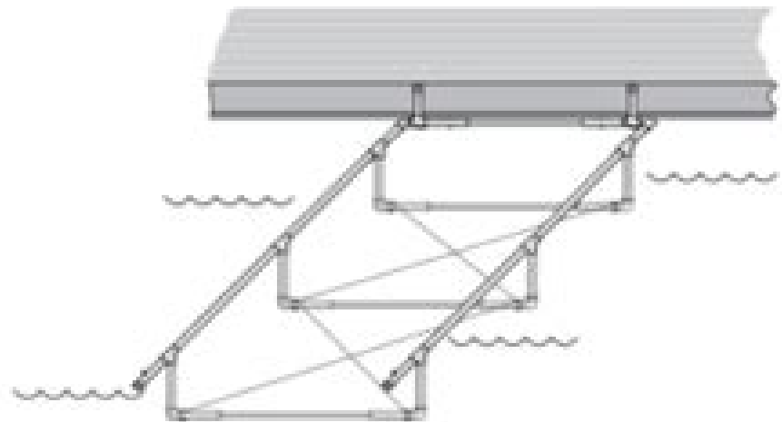
Floating dock with our Super Full Frame kit front mounted on the dock.
