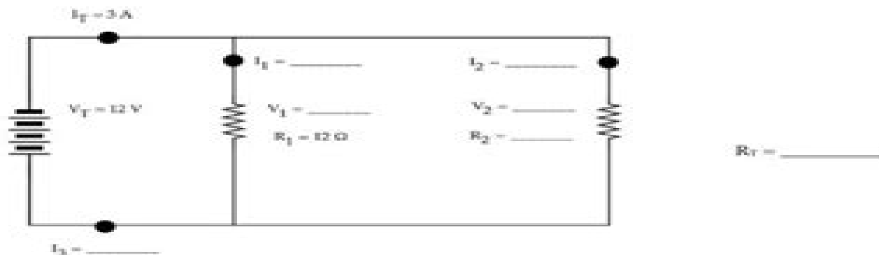
Circuit.2
