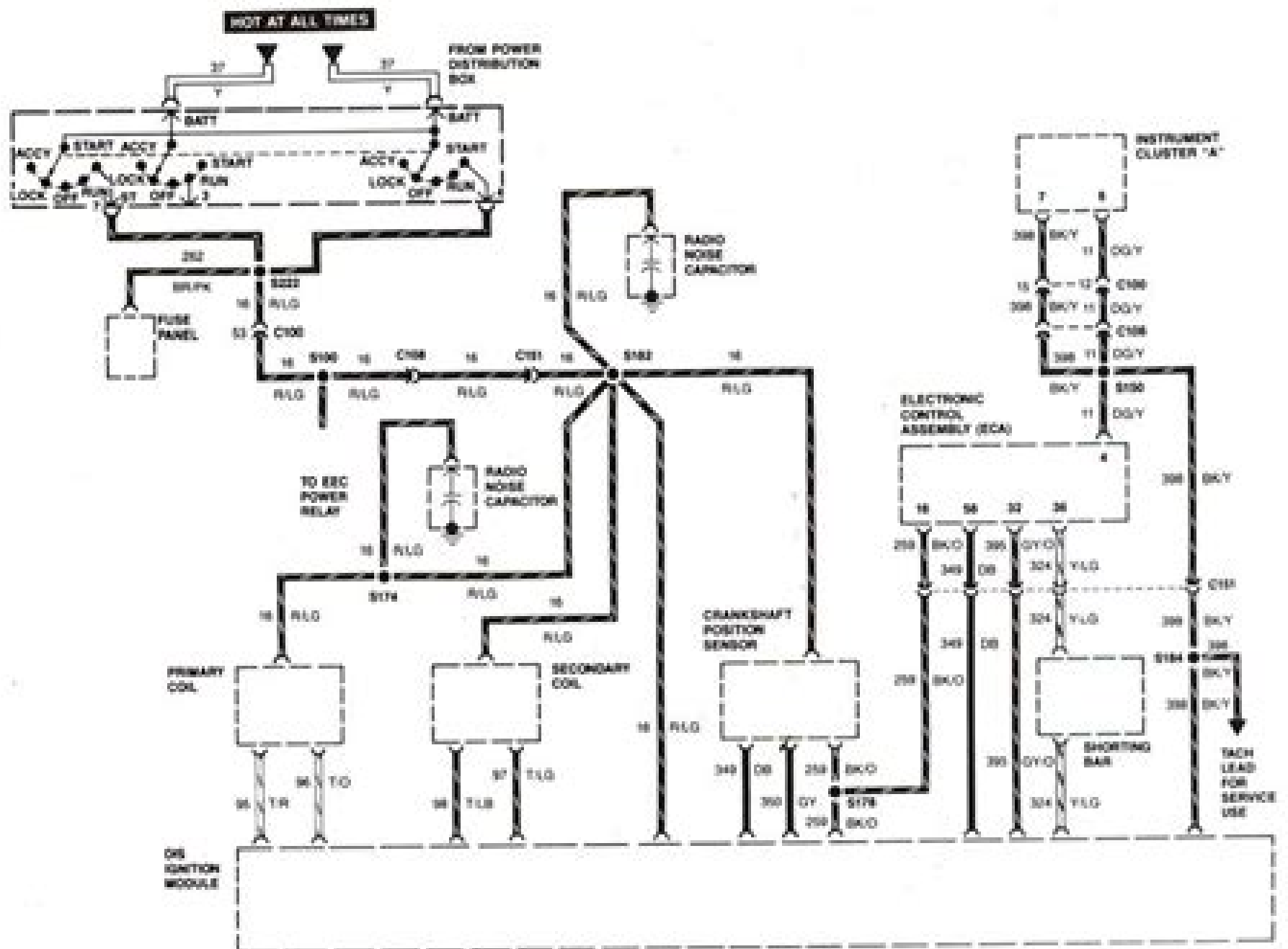
Ignition system – 1989 2.3L engine
