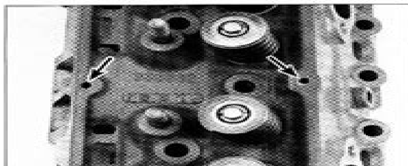
1.5 Most 1969 and later cylinder heads have valve cover bolts that are directly opposite each other
