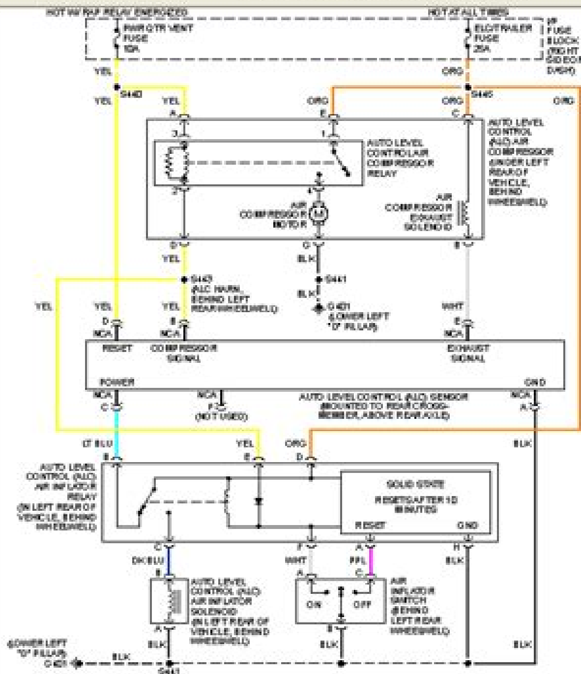
Fig. 14: Electronic Suspension Circuit, W/ Inflator
