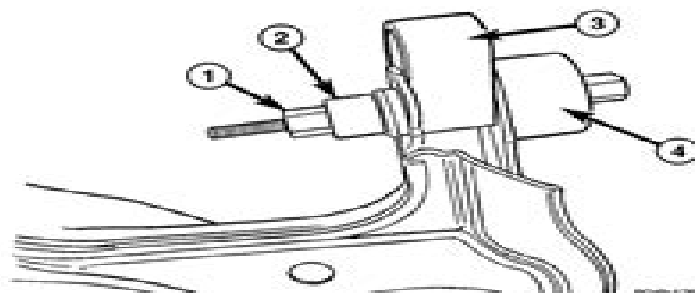
Fig. 7 SMALL LOWER CONTROL ARM BUSHING - REMOVAL
