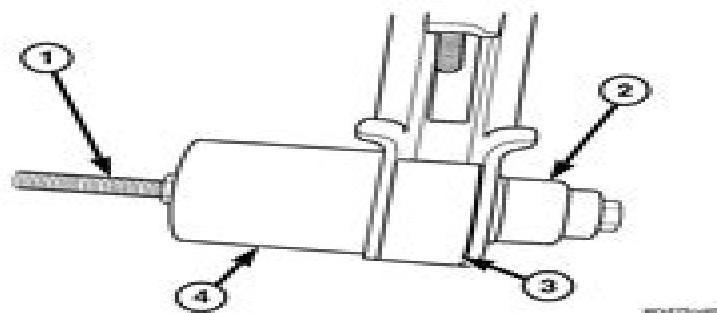
Fig. 5 TORSION BAR CROSS MEMBER BUSHING - REMOVAL
