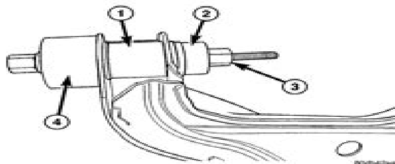
Fig. 6 LARGE LOWER CONTROL ARM BUSHING - REMOVAL
