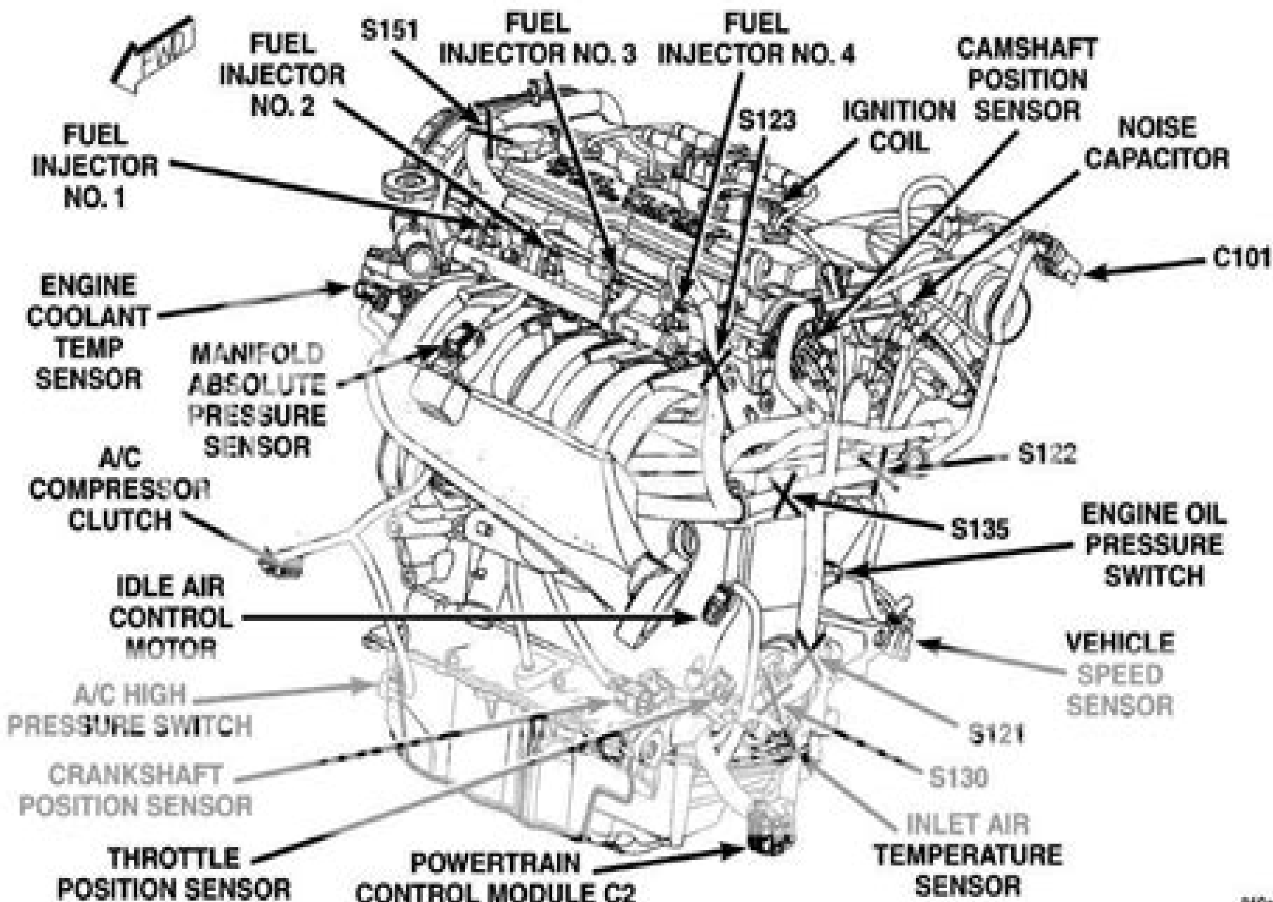
Fig. 15 ENGINE (LEFT FRONT) (2.4L TURBO) — LHD
