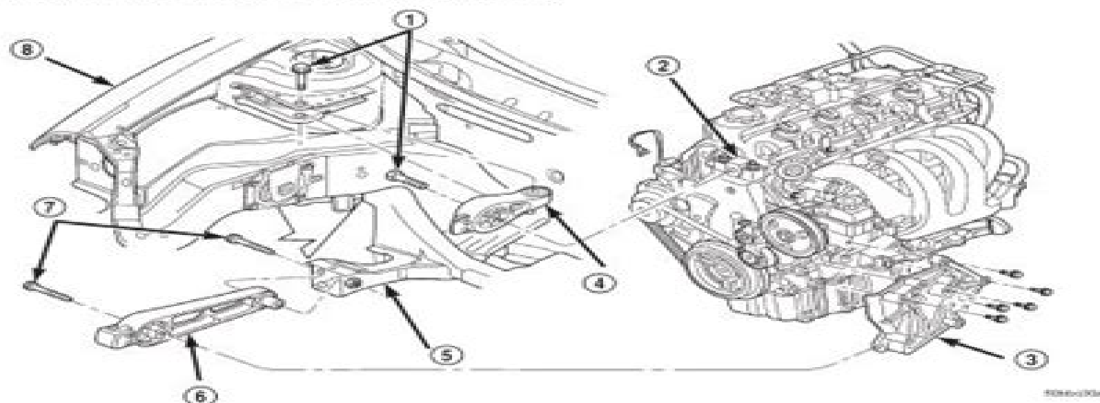
Fig. 10 Torque Struts—Upper and Lower
