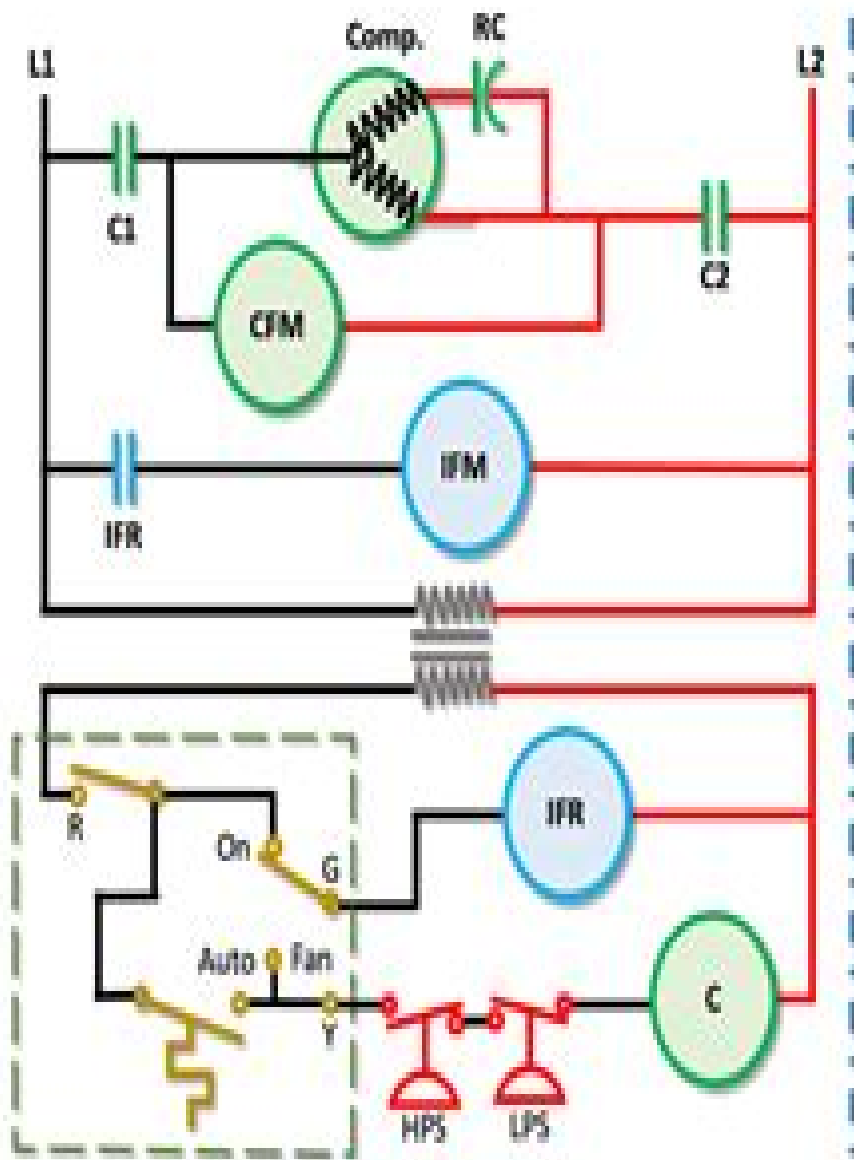
Schematic Diagram (Ladder Diagram)
