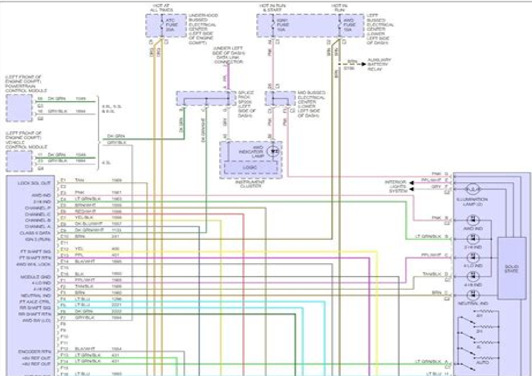
Fig 2: Transfer Case Circuit, Electronic
