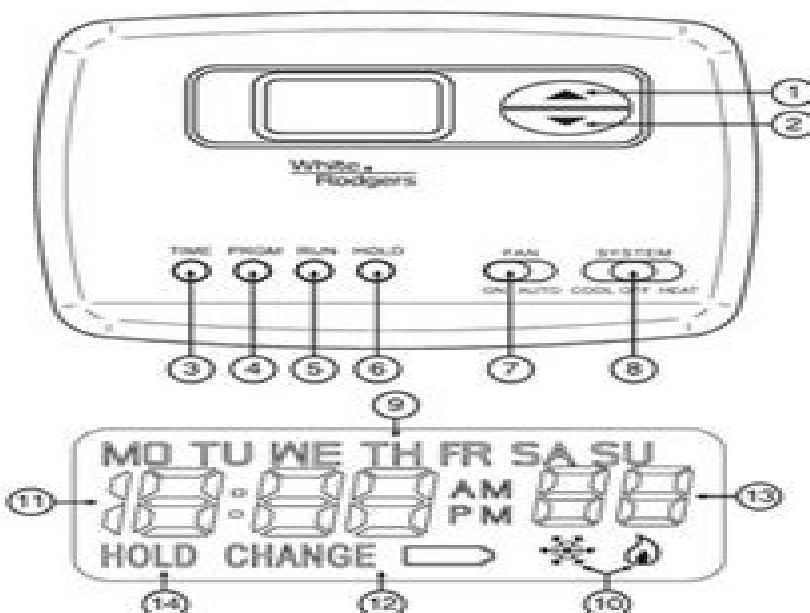
Figure 6. Thermostat display, buttons, and switches
