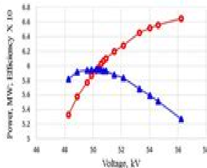
Figure 5: The efficiency (triangular) and RF power production (circle) in saturation at 3.003 GHz as functions of high voltage.
