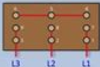
230-V connection
