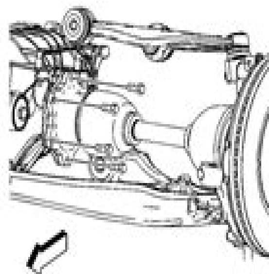
Fig. 3. View Of Wheel Drive Shaft Retaining Bolt Courtesy of GENERAL MOTORS CORP.
