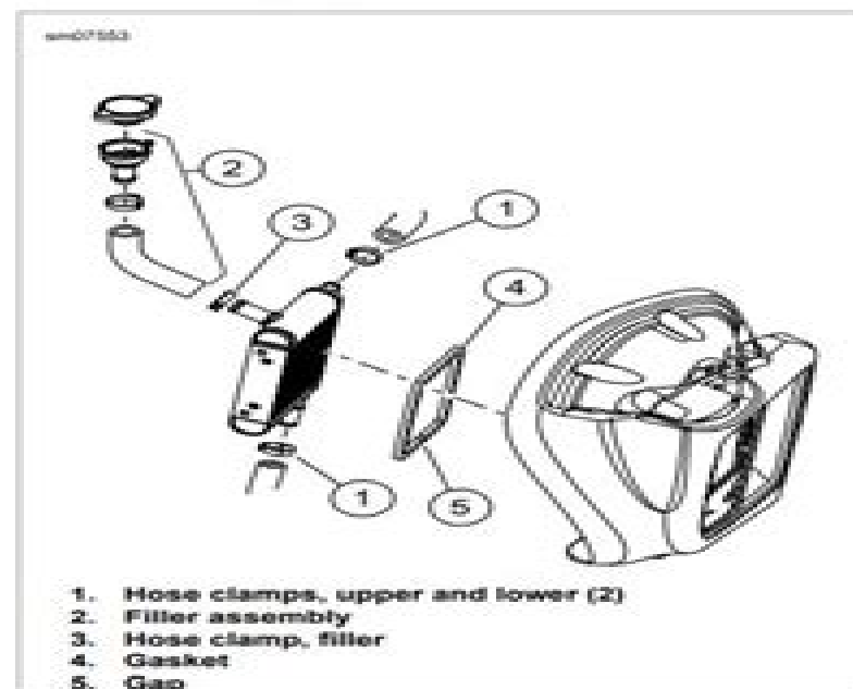
Figure B-10. Radiator
