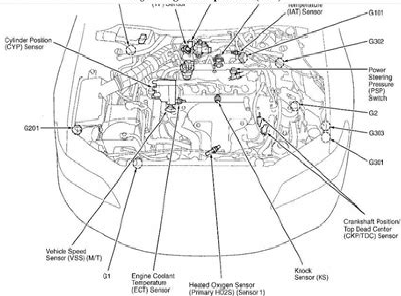
Fig. 1: Engine Compartment (2.3L)
