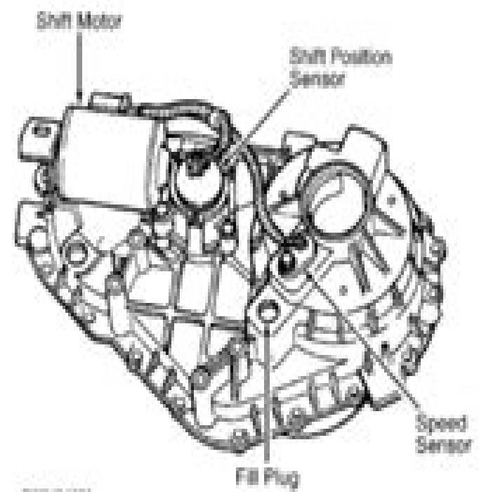
Fig. 1: Identifying Model 4405 Transfer Case Courtesy of Ford Motor Co.
