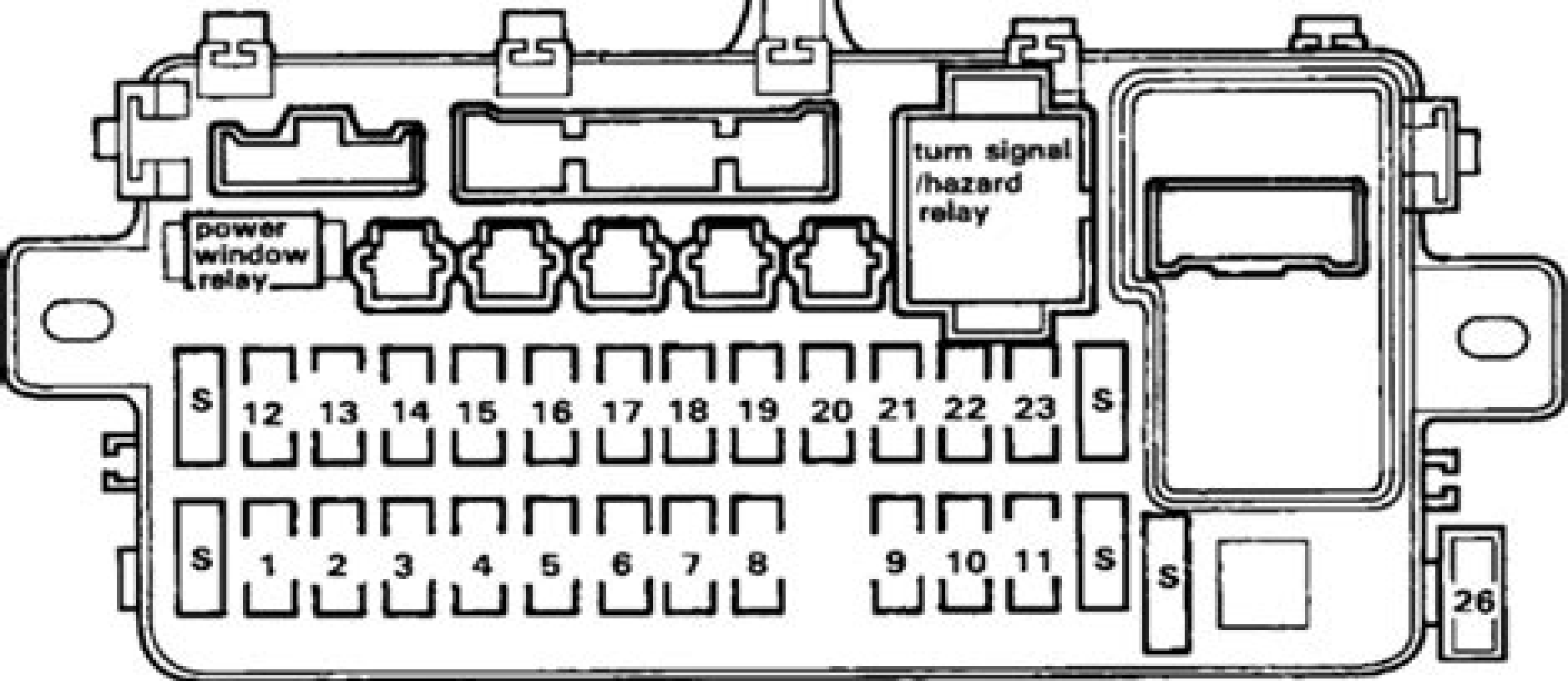
SRS FUSE BLOCK
