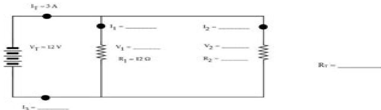
Circuit.2
