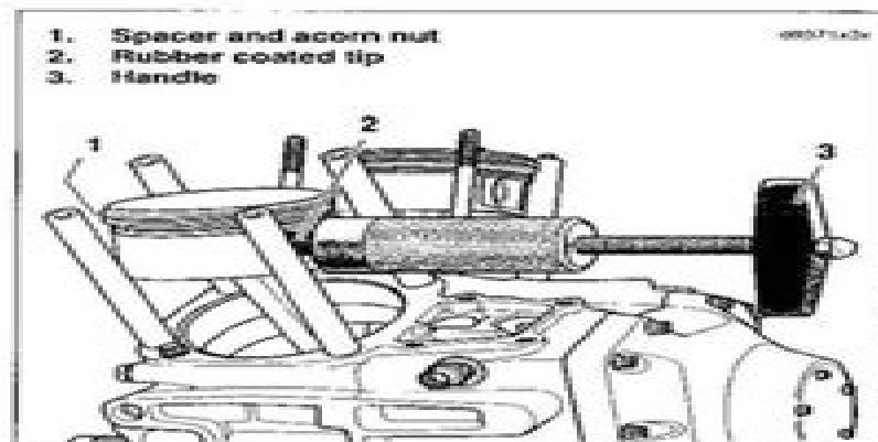
Figure 3-28. Piston Pin Remover (Part No. HD-42320-A)
