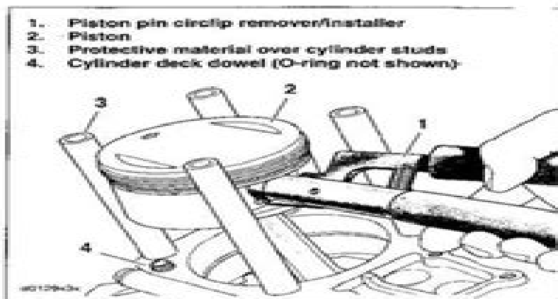
Figure 3-27. Piston Pin Circlip Removal (Part No. HD-42317)
