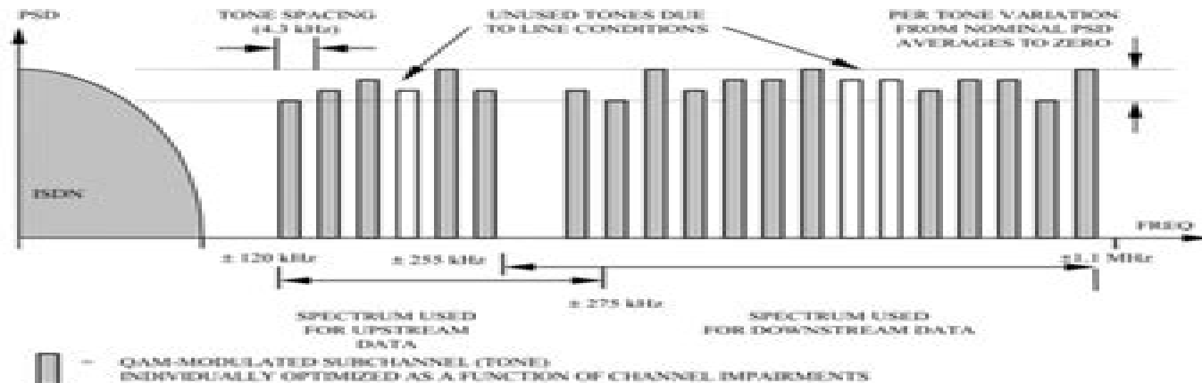
Figure 5 - DMT Spectrum Used in ADSLx above ISDN Modem
