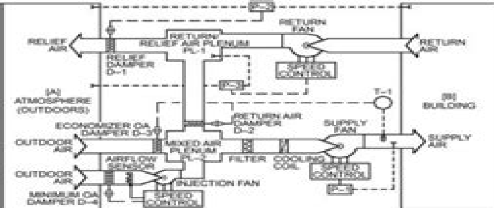
A. ECONOMIZER CYCLE WITH RETURN FAN
