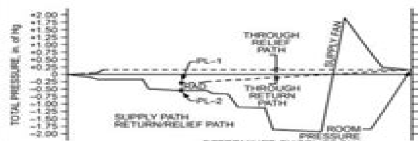
C. ECONOMIZER CYCLE WITH GRAVITY OR MOTORIZED RELIEF DAMPER
