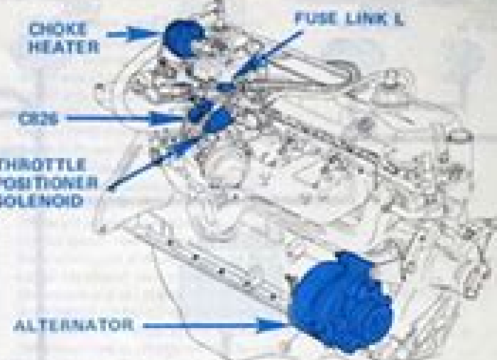
Figure 2 - RH Side of Heavy Duty 4.9L Engine
