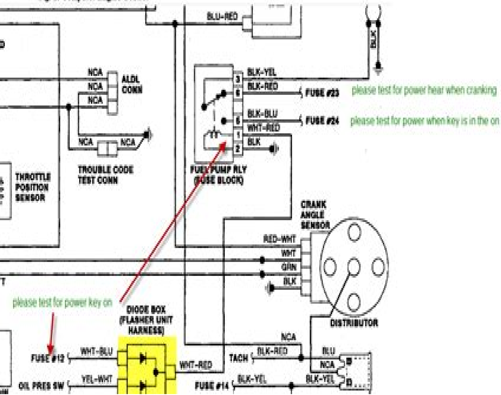
Fig. 2: Computer Engine Control
