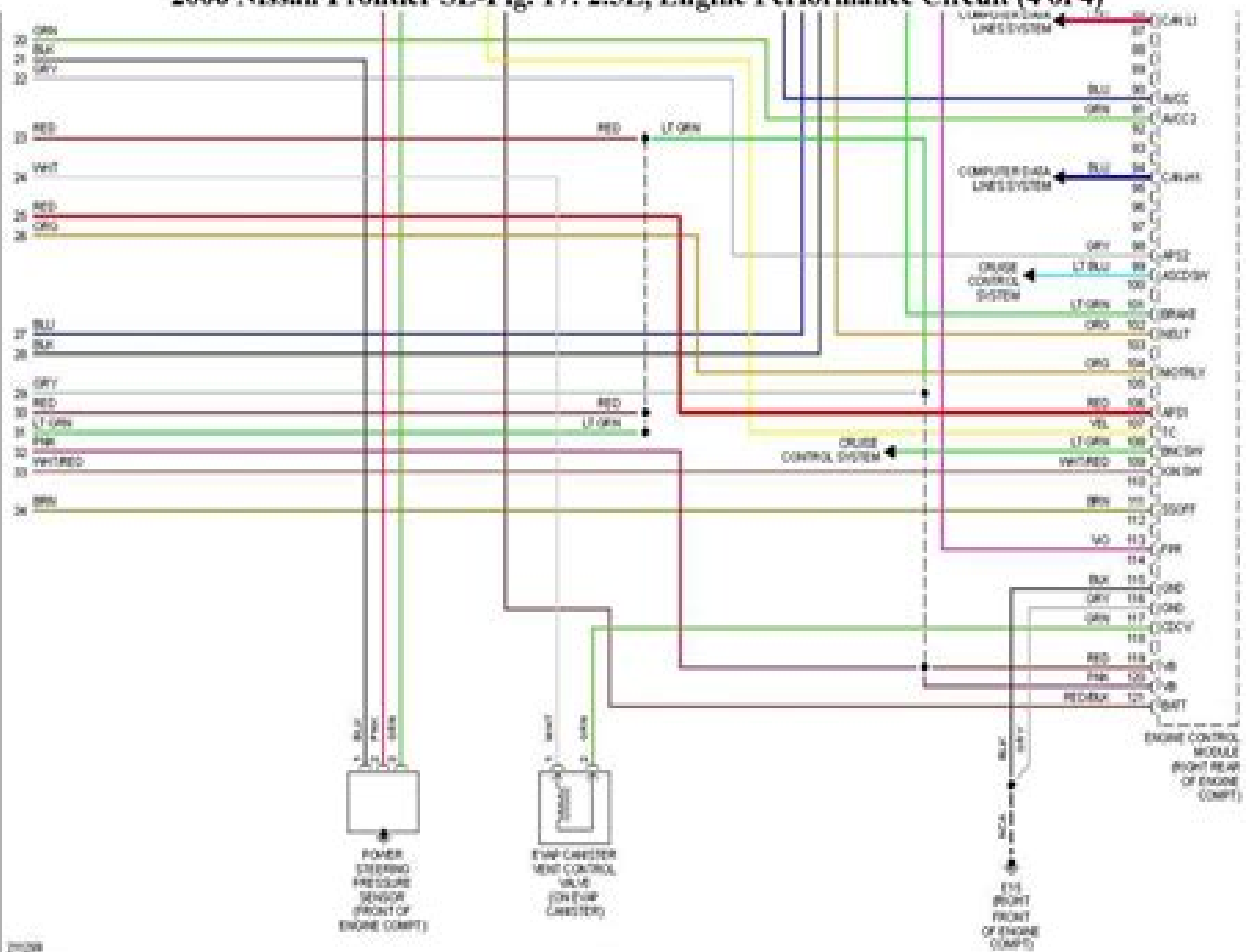
2006 Nissan Frontier SE-Fig. 17: 2.5L, Engine Performance Circuit (4 of 4)
