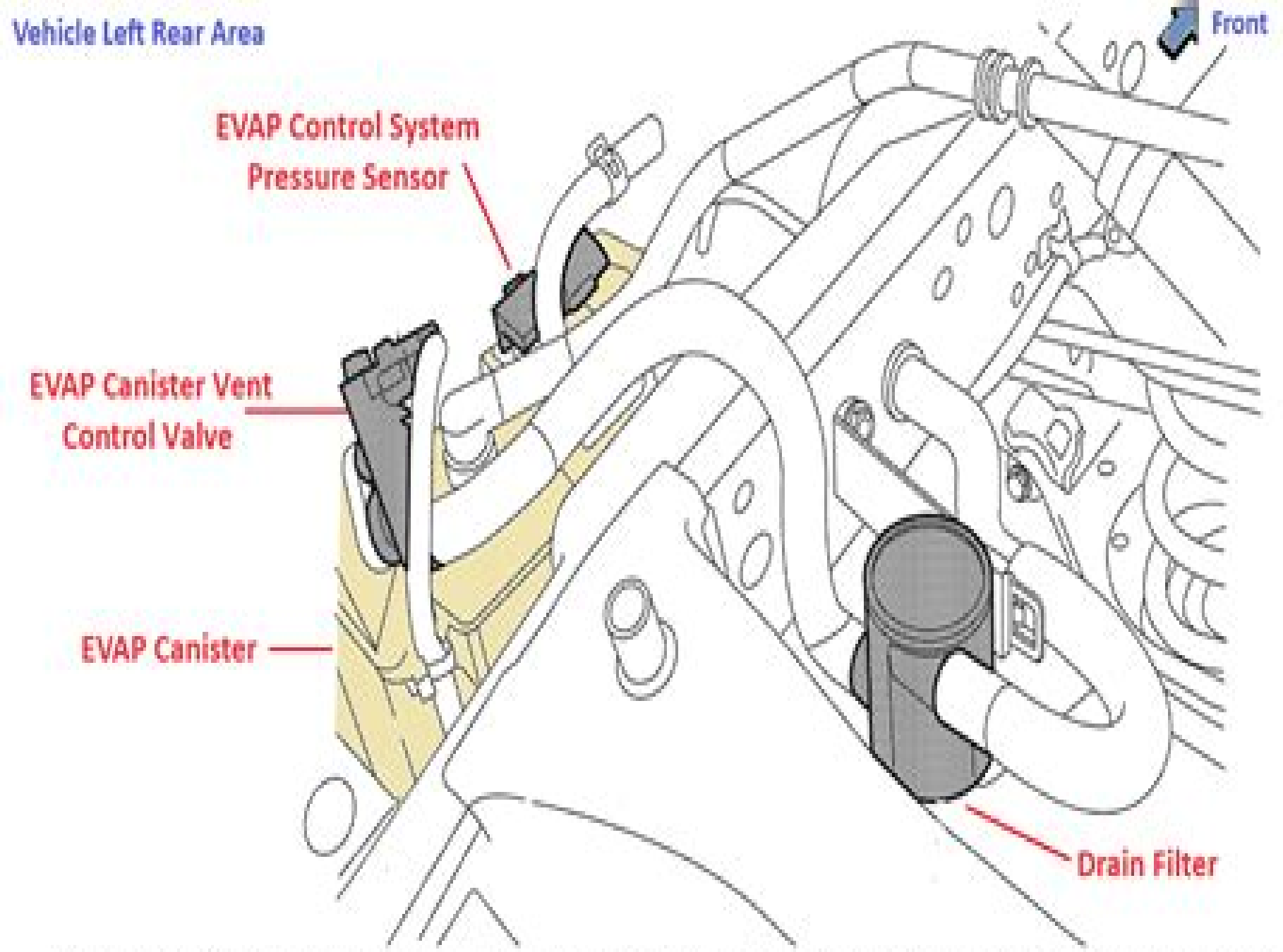
Nissan Pathfinder EVAP Canister Vent Control Valve - EVAP Control System Pressure Sensor
