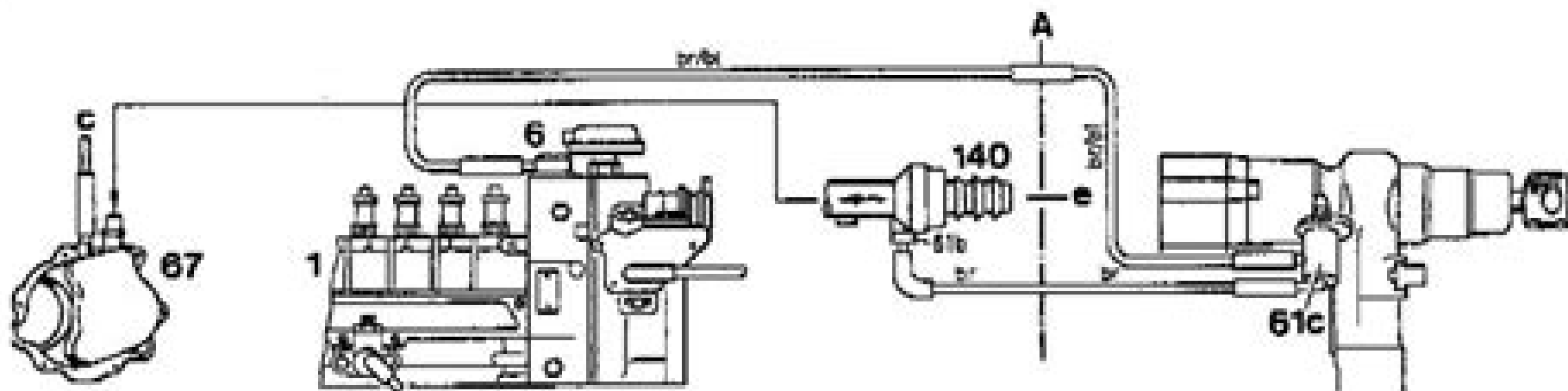
Vacuum line routing
