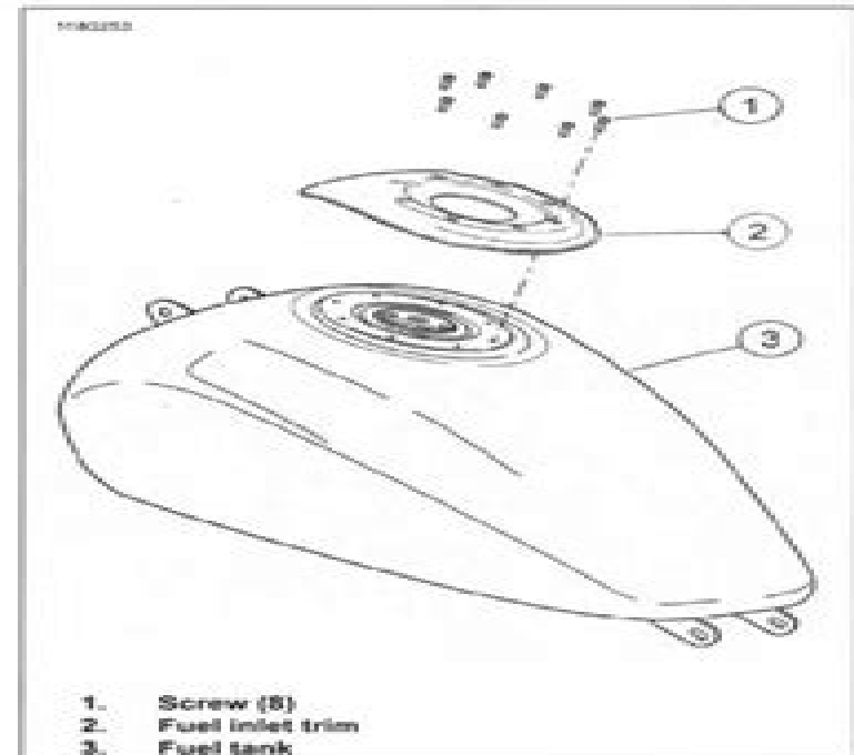
Figure 6-17. Fuel Fill Port
