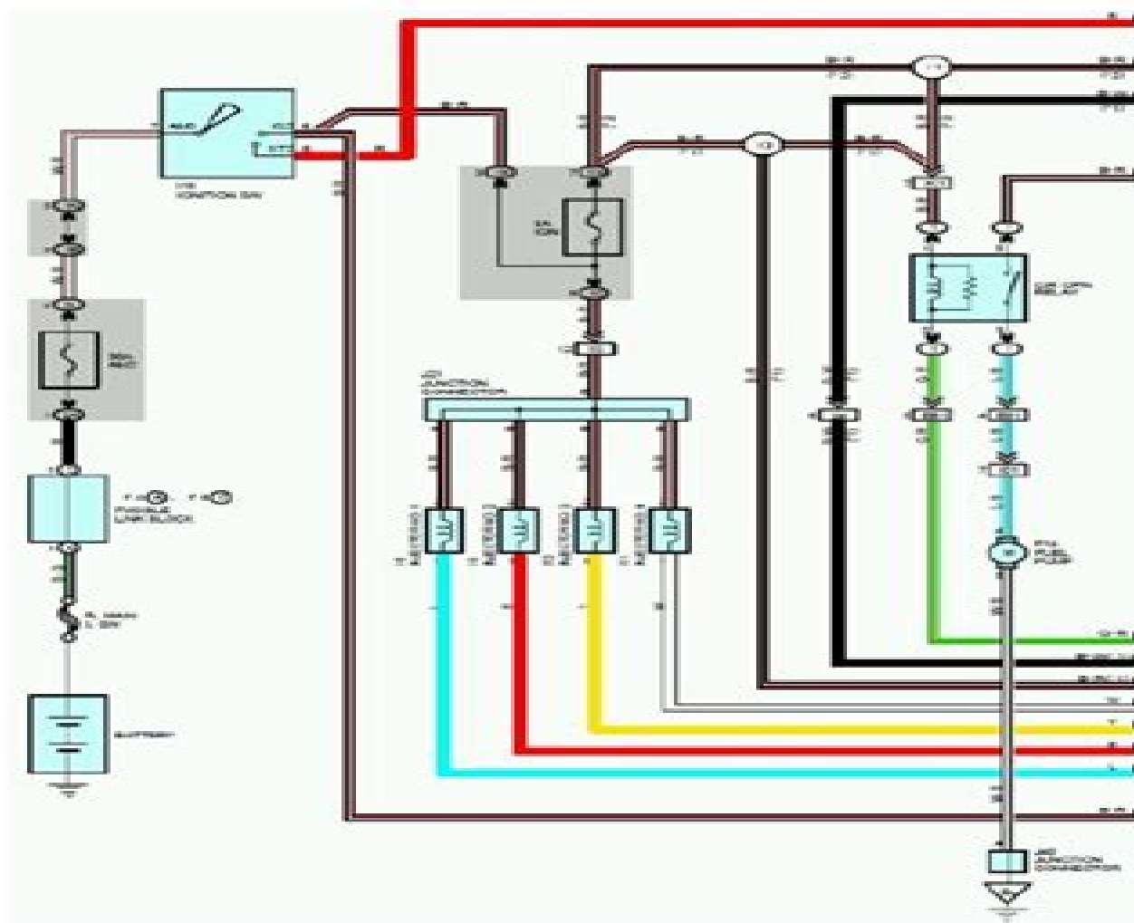
Engine Control (1 Of 6)
