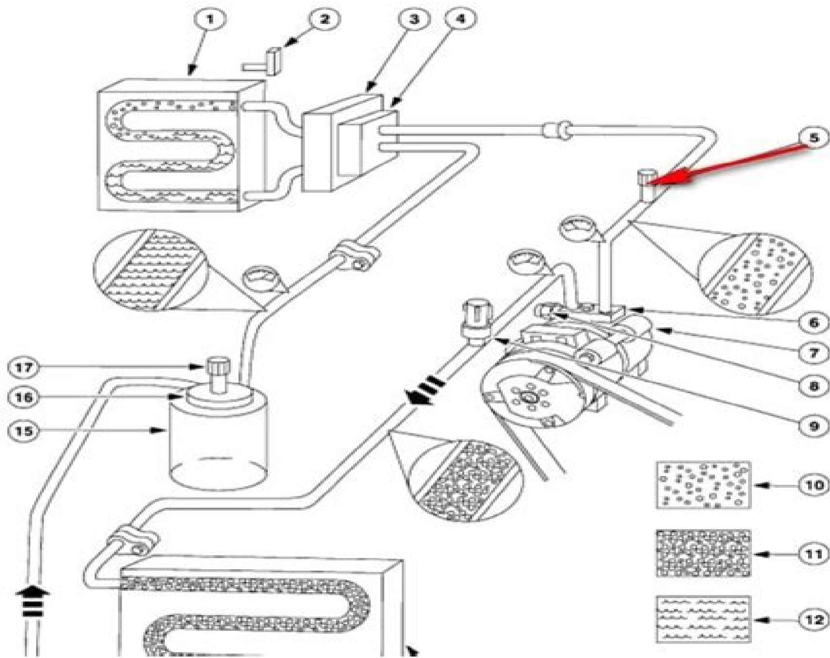
Clutch Cycling Thermostatic Expansion Valve Type Refrigerant System
