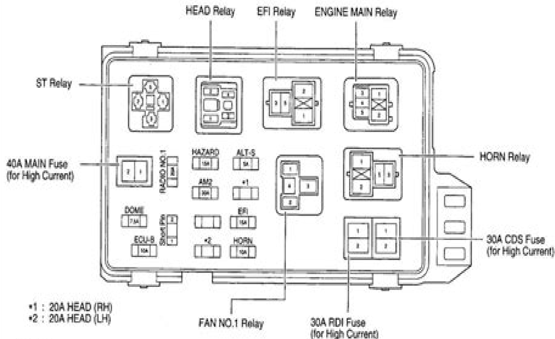
Fig 9: Identifying Engine Room J/B No. 2 Components
