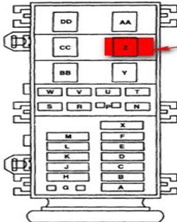
POWER DISTRIBUTION BOX
