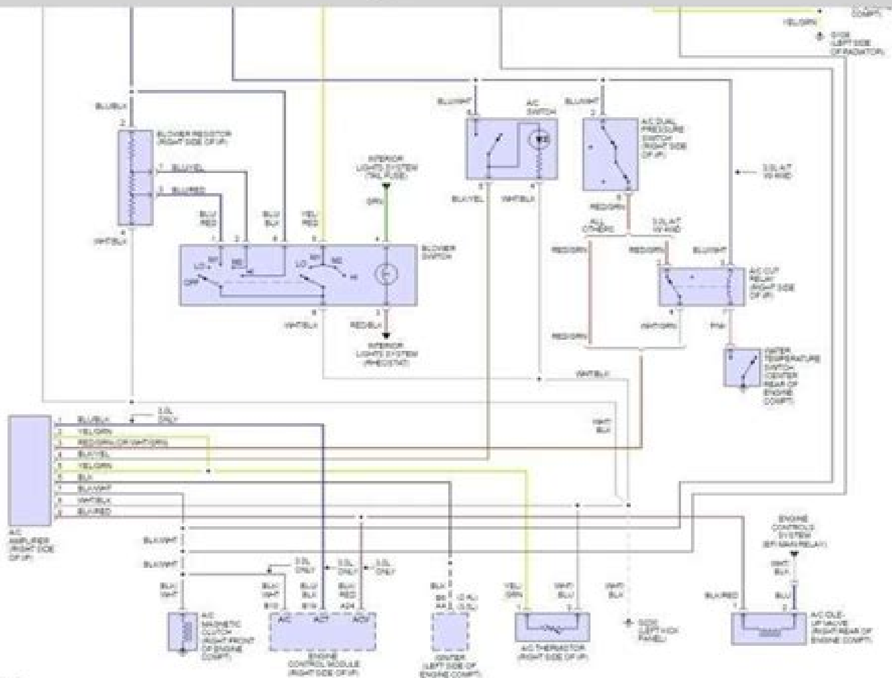
Fig 1: A/C Circuit
