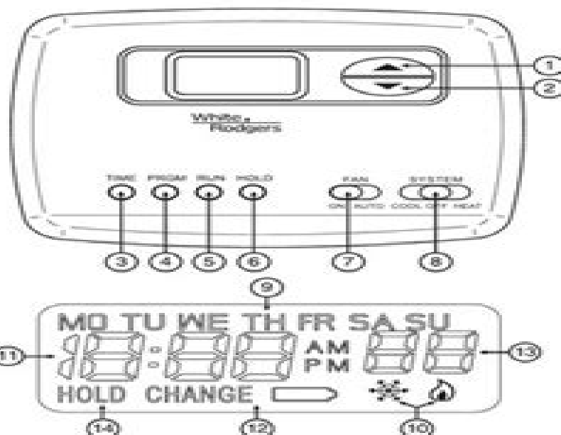
Figure 6. Thermostat display, buttons, and switches
