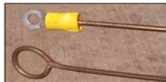
Fig 22.97 — Alternate methods for terminating element and radial tips on the simple groundplane antenna. See text. [Photo by KBCH]
