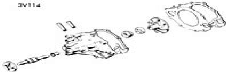
260", 289", 302", 351" W ENGINES WATER PUMP
