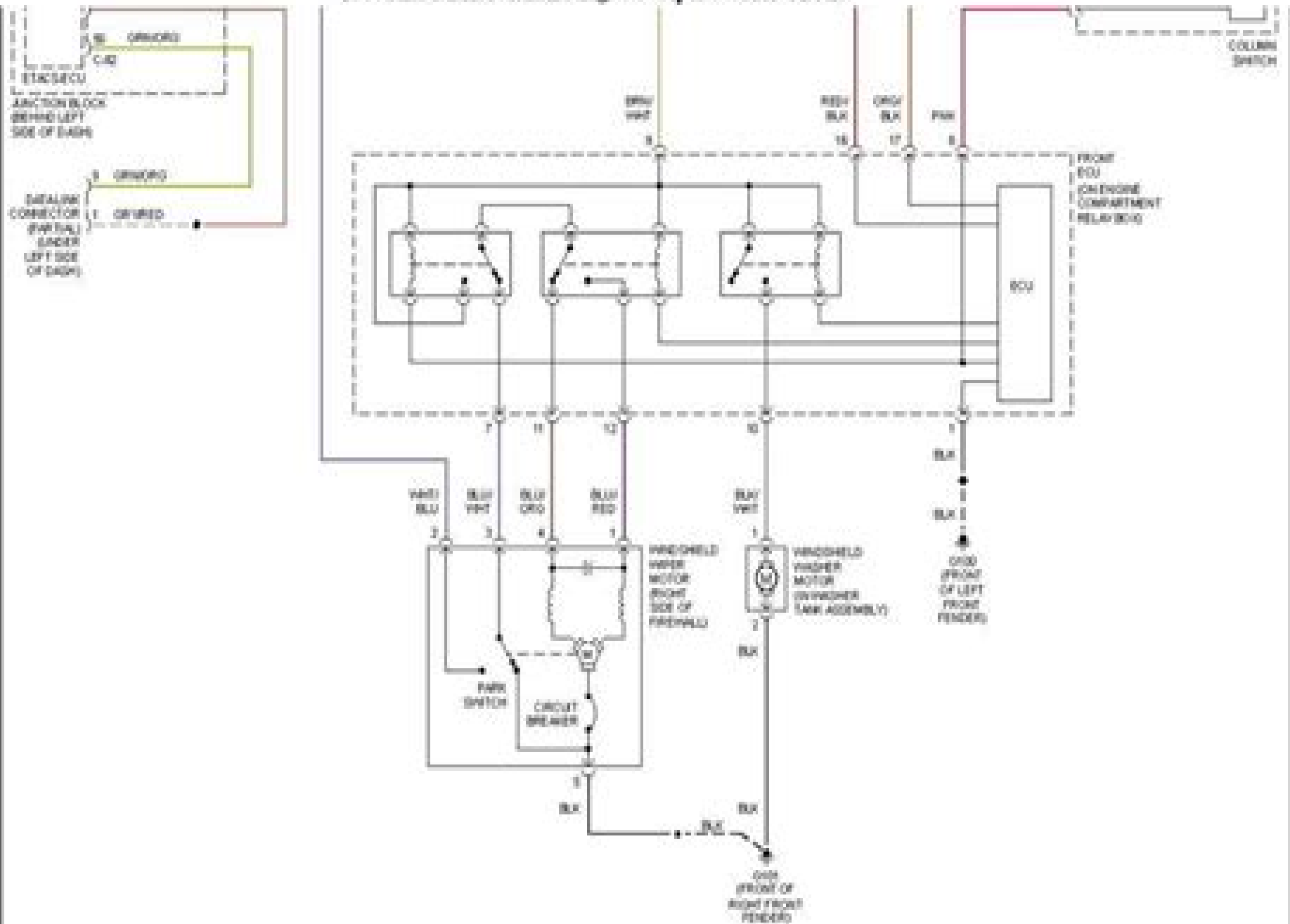
2006 Mitsubishi Galant ES Fig. 46: Wiper-Washer Circuit
