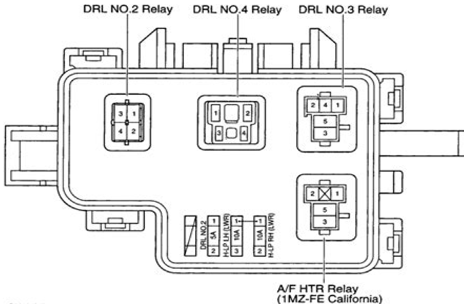
Fig 14: Identifying Engine Room R/B No. 2 Components (With Daytime Running Lights)
